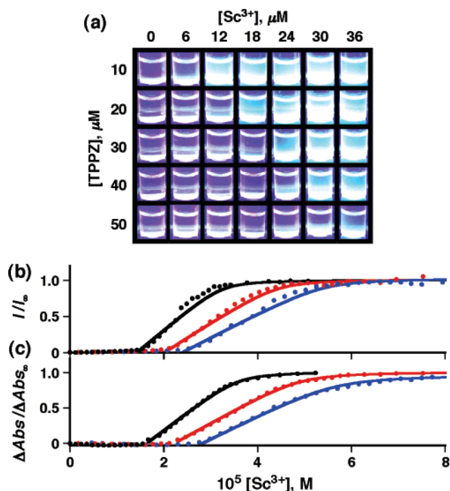
Figure 8. (a) Change in visible fluorescence of MeCN solutions of TPPZ ( 1.0 \times 10^{-5} to 5.0 \times 10^{-5} M) in the presence of Sc^{3+} [ (0-3.6) \times 10^{-5} M]. Plots of (b) I/I_\infty at 453 nm and (c) \Delta Abs/\Delta Abs_\infty [= (A - A_0)/(A_\infty - A_0) ] at 303 nm vs [Sc^{3+}] for the titration of TPPZ [ 3.4 \times 10^{-5} M (black closed circles), 4.7 \times 10^{-5} M (red closed circles), and 5.7 \times 10^{-5} M (blue closed circles)] by Sc^{3+} in MeCN at 298 K.
